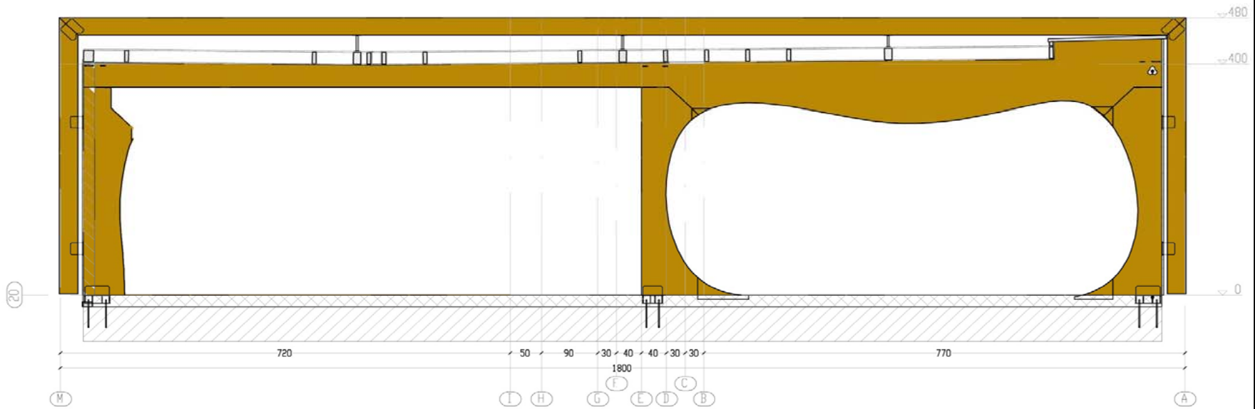
FIGURE 02 SECTION
